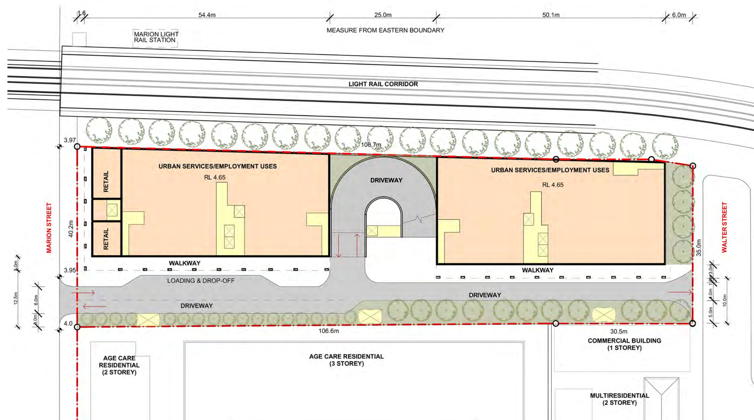
LEVEL 1- GROUND FLOOR
